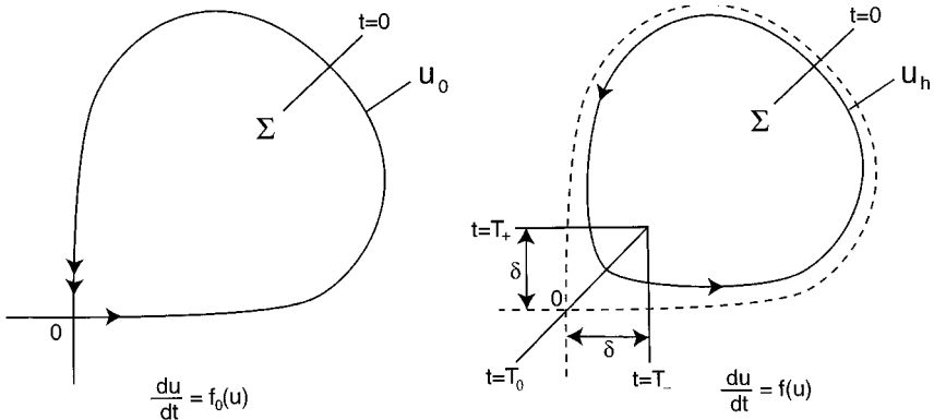
Fig. 5. Homoclinic and quasi-homoclinic orbits.
