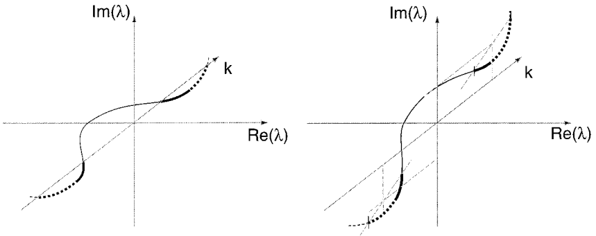
Fig. 1. Growth rate versus wave number, for \mu < 0 and D_{1,1} < 0 ; left corresponds to case (a) and right to case (b) (dotted lines are for terms of order higher than k^2 ).
