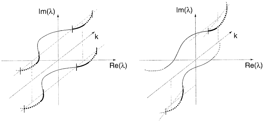
Fig. 2. Growth rate vs wave number for Hopf instability with a first order spatial derivative term (Dotted line are for higher order terms). Figure on the left corresponds to case (a), when D_{1,1} + D_{2,2} < 0 , and figure on the right corresponds to case (b), when C_{2,1} - C_{1,2} < 0 .
