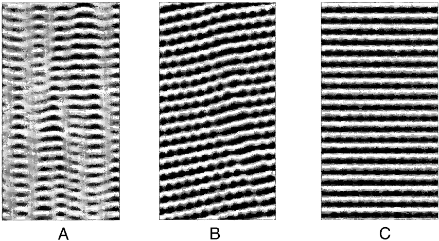
Fig. 9. Numerical simulation of Eqs. (14) and (15).
