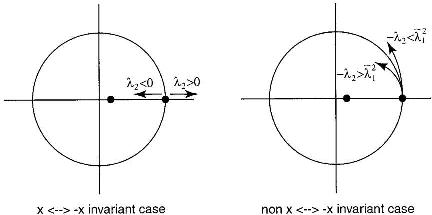
Fig. 3. Behavior of \lambda(k) for |k| small.
