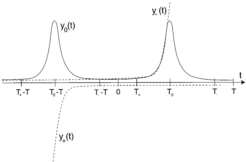
Fig. 7. Behaviors of y_0(\cdot) , y_+(\cdot) , and y_-(\cdot) on \mathbf{R} .
