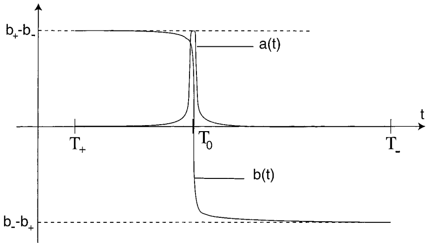
Fig. 6. Behavior of a(t) and b(t) for t \in [T_+; T_-] .
