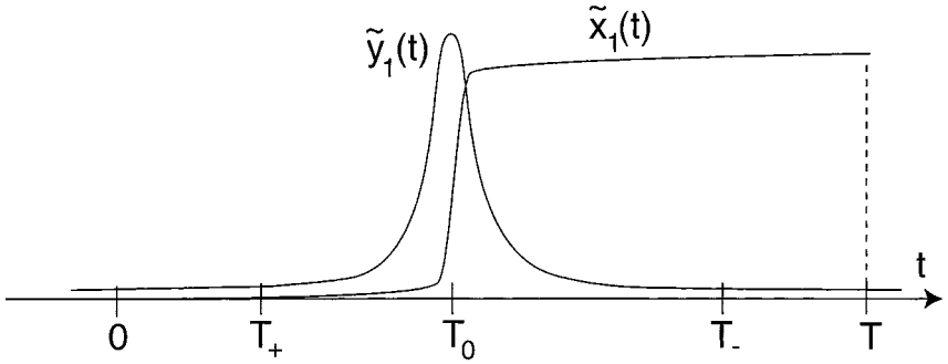
Fig. 8. Behaviors of \tilde{x}_1(t) and \tilde{y}_1(t) for t \in [0; T] .
