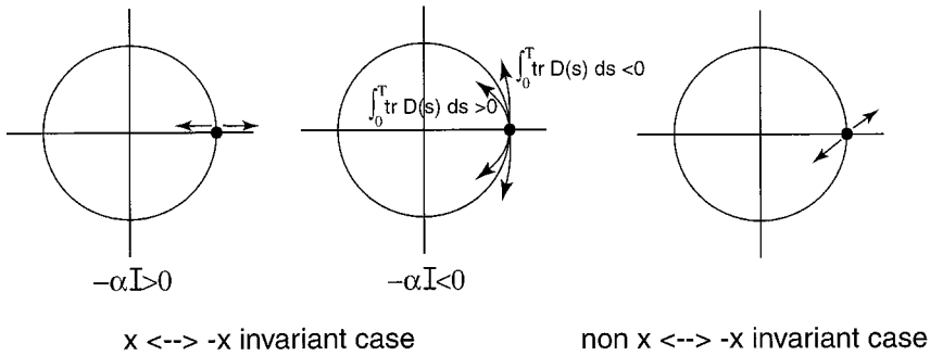
Fig. 4. Behavior of the two eigenvalues of \Phi_k(T) for |k| small, at a saddle-node of cycles.
